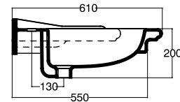
Royal Lavabo cm 110 Washbasin cm 110 Lavabo cm 110 COD. 40129
