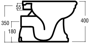
Royal Vaso scarico P Wc bowl wall trap Inodoro salida H COD. 27003
