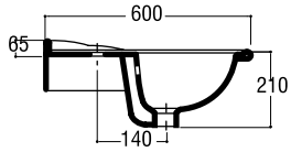
Royal Lavabo Angolo Corner Washbasin Lavabo Angular COD. 30353
