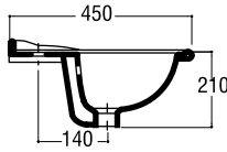
Royal Lavabo incasso cm 56 Built in washbasin cm 56 Lavabo encastre cm 56 COD. 30354
