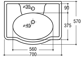
Royal Lavabo cm 70 Washbasin cm 70 Lavabo cm 70 COD. 27021
