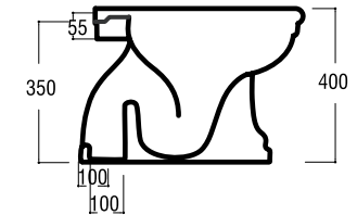
Royal Vaso scarico S Wc bowl floor trap Inodoro salida V COD. 27004
