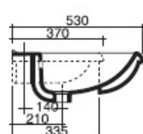
Hola Lavabo cm 56 Wash basin cm 56 Lavabo cm 56 COD. 29037
