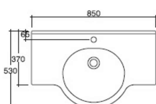
Hola Lavabo cm 85 Wash basin cm 85 Lavabo cm 85 COD. 29036
