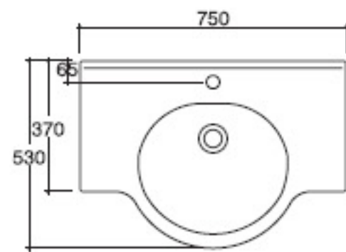
Hola Lavabo cm 75 Wash basin cm 75 Lavabo cm 75 COD. 29043
