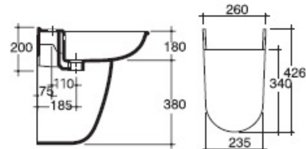
Hola Semicolonna Half Pedestal Semipedestal COD. 29031
