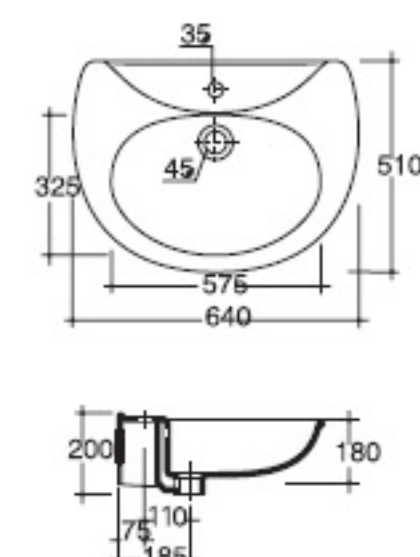
Hola Lavabo cm 64 Washbasin cm 64 Lavabo cm 64 COD. 29020
