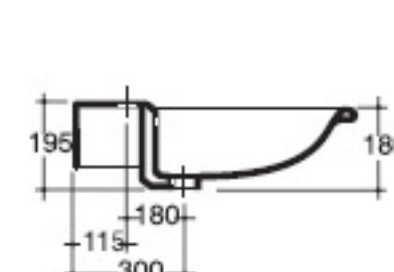
Hola Lavabo cm 56 Wash basin cm 56 Lavabo cm 56 COD. 29037
