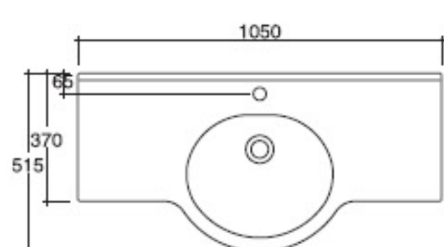
Hola Lavabo cm 105 Wash basin cm 105 Lavabo cm 105 COD. 29035
