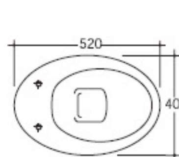
Hola Vaso scarico P Wc bowl wall trap Inodoro salida H COD. 29003
