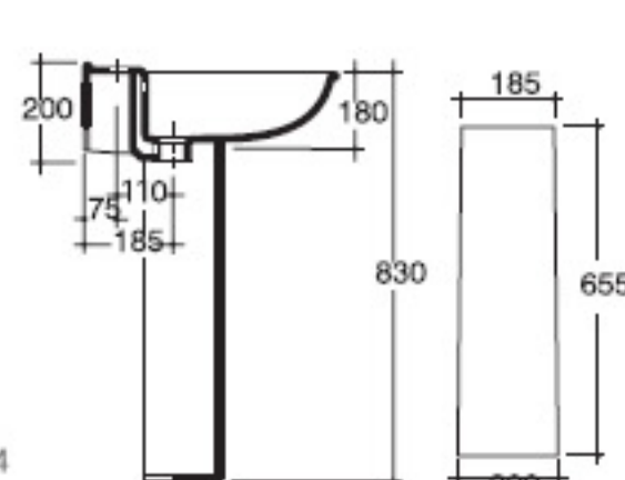
Hola Colonna Pedestal Pedestal COD. 29030
