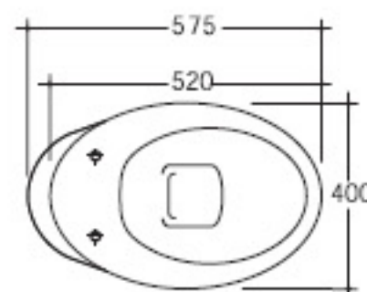
Hola Vaso scarico S Wc bowl floor trap Inodoro salida V COD. 29004
