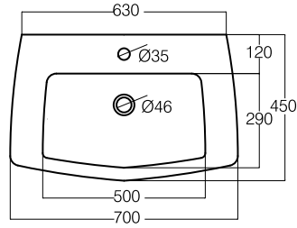
Oceano Lavabo 70 Washbasin cm 70 Lavabo cm 70 COD. 30329
