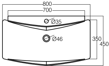
Oceano Lavabo 80 Washbasin cm 80 Lavabo cm 80 COD. 30330
