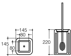
D-Style Portascopino Toilet brush holder Escobillero COD. 40026 COD. 40044 COD. 40045 COD. 40046 COD. 40047
